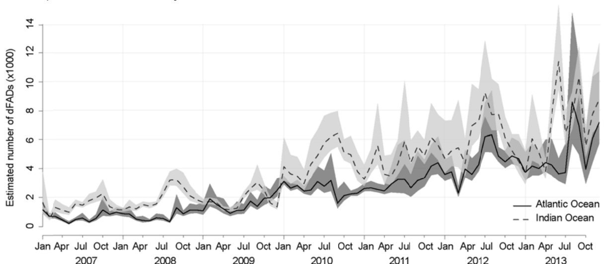
Figure 3. Estimation of the total number of GPS buoy-equipped dFADs in the main purse seine fishing grounds of the Atlantic (solid line) and Indian (dashed line) oceans, at the end of each month (2007-2013). Grey areas represent the 95% Confidence Intervals (CI).
